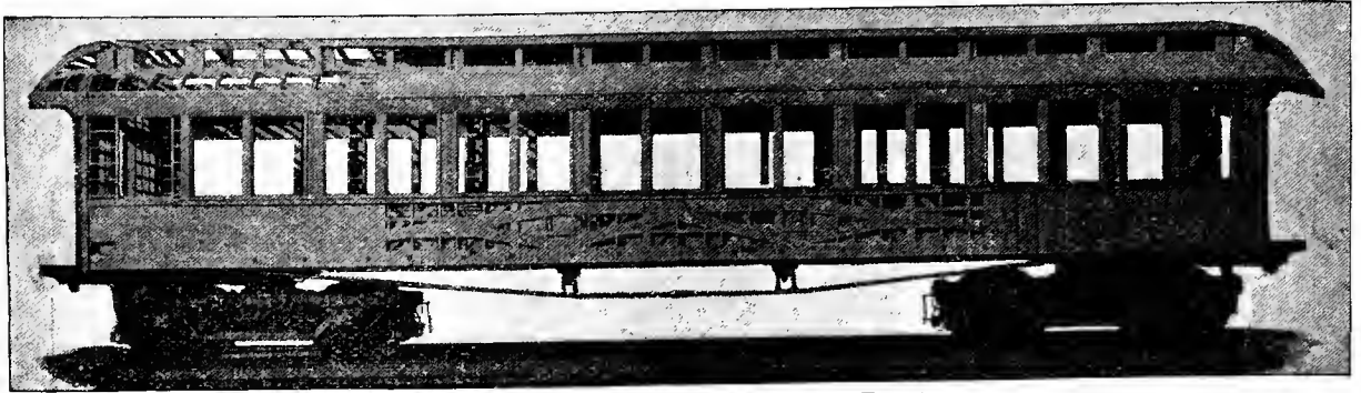
Fig. 531. Side View, showing Truss and Roof Framing.
